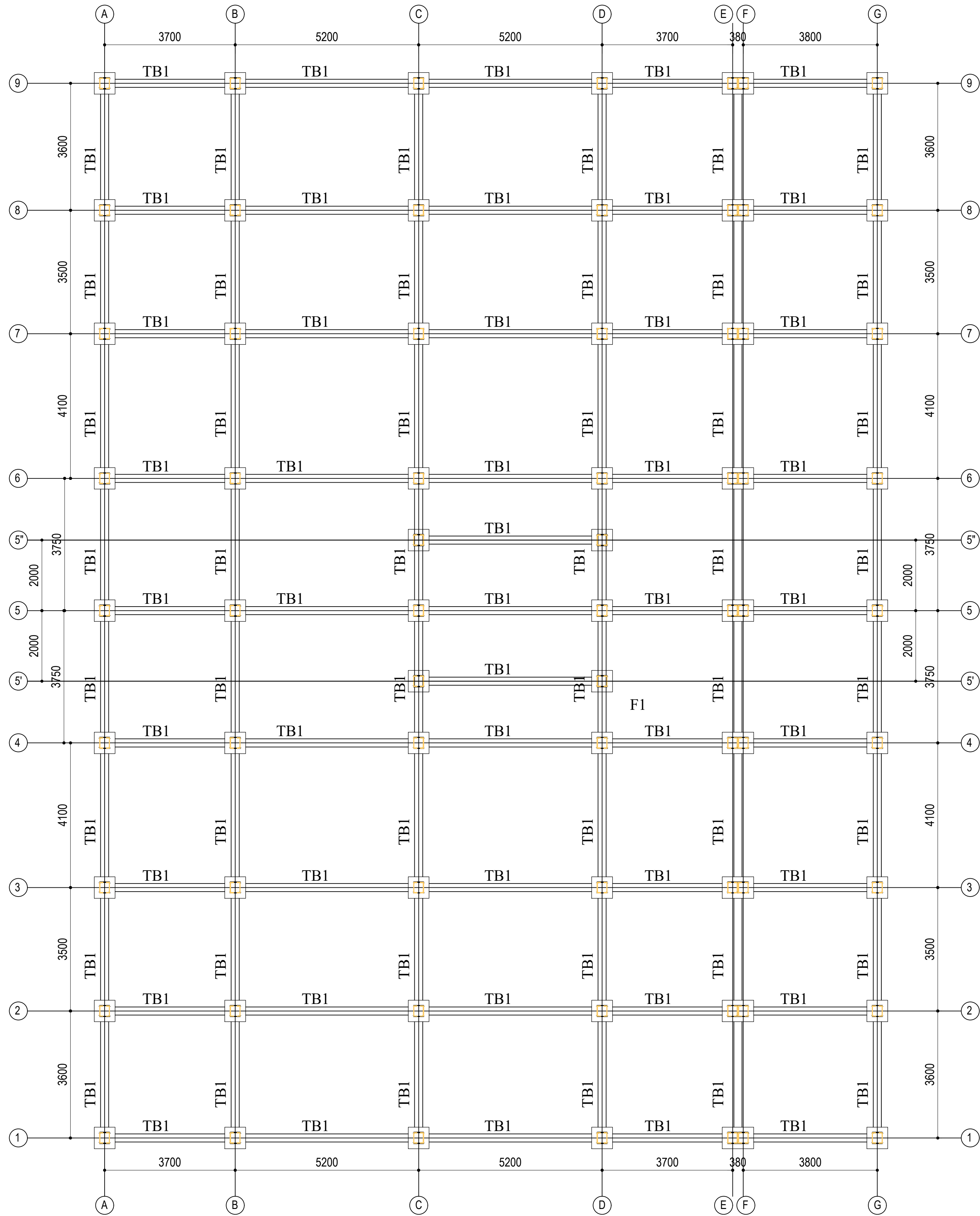
Tie Beam Layout Plan
