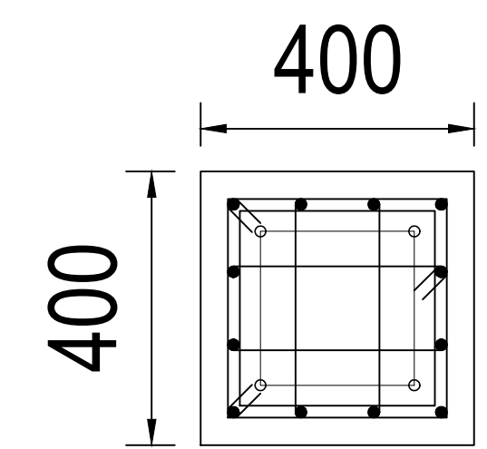
PEDESTAL DETAIL OF FOUNDATION-F1
