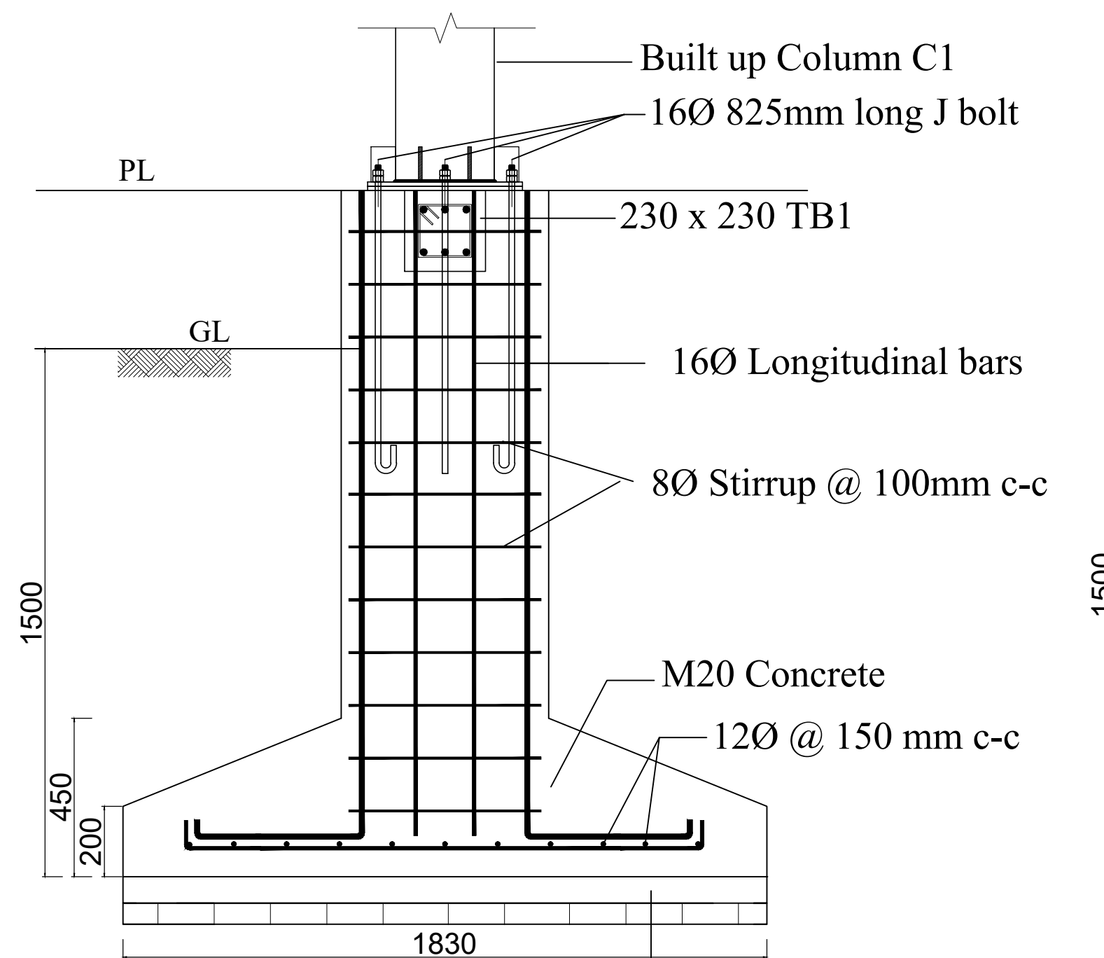
SECTION-F2a COLUMN FOUNDATION DETAILS
