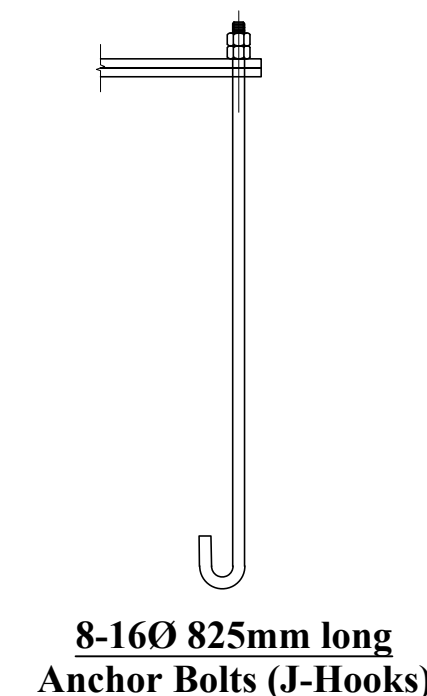
PEDESTAL DETAIL OF FOUNDATION-F1
