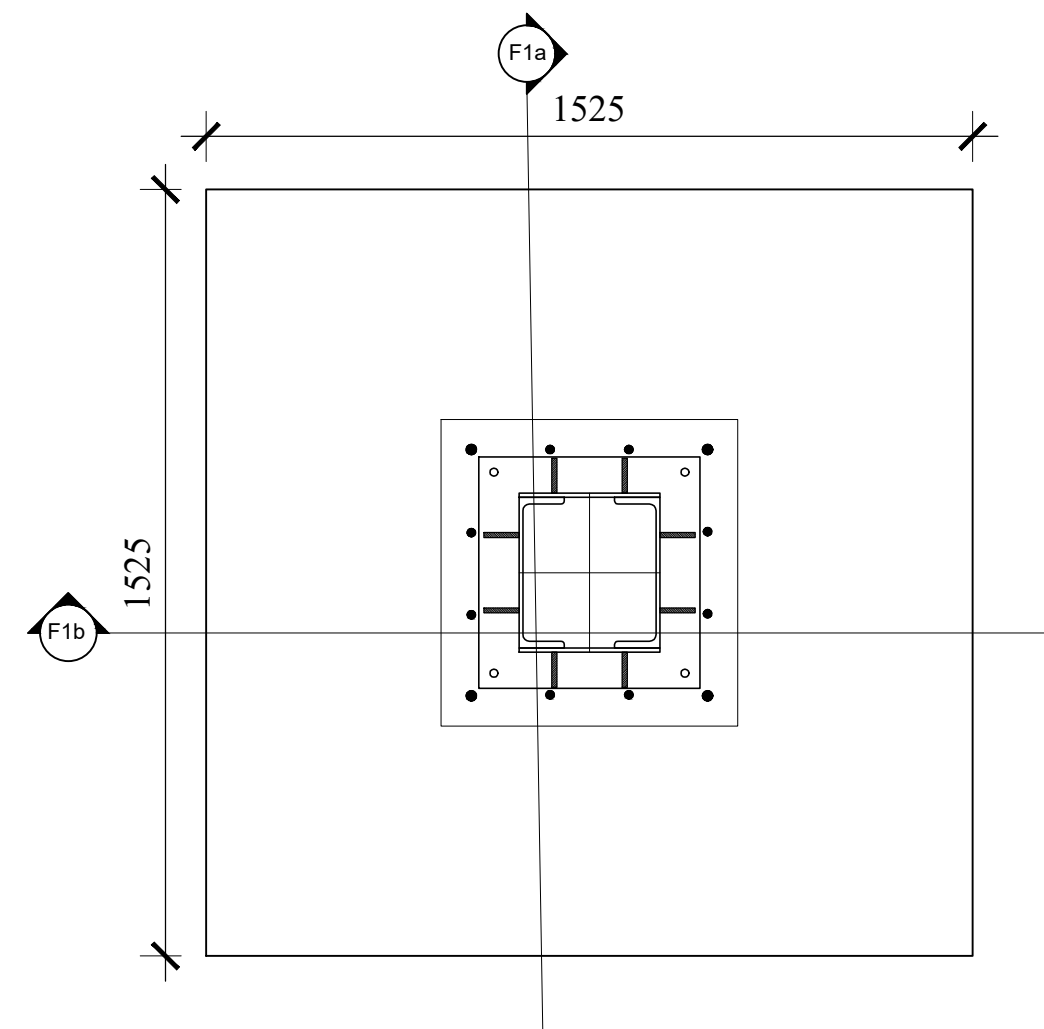
FOUNDATION-F1
