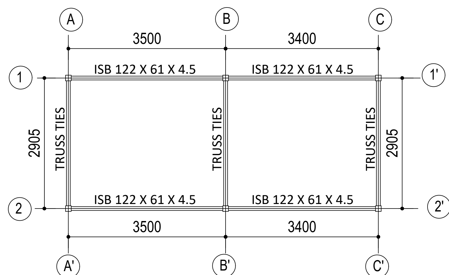
FLOOR BEAM LAYOUT PLAN
