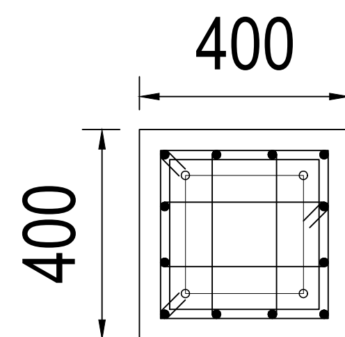
PEDESTAL DETAIL OF FOUNDATION-F1
