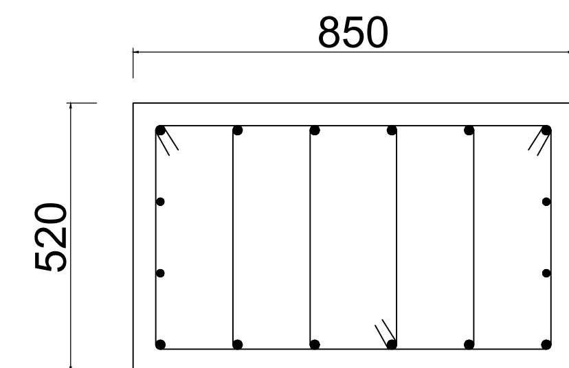
PEDESTAL DETAIL OF FOUNDATION-F3
