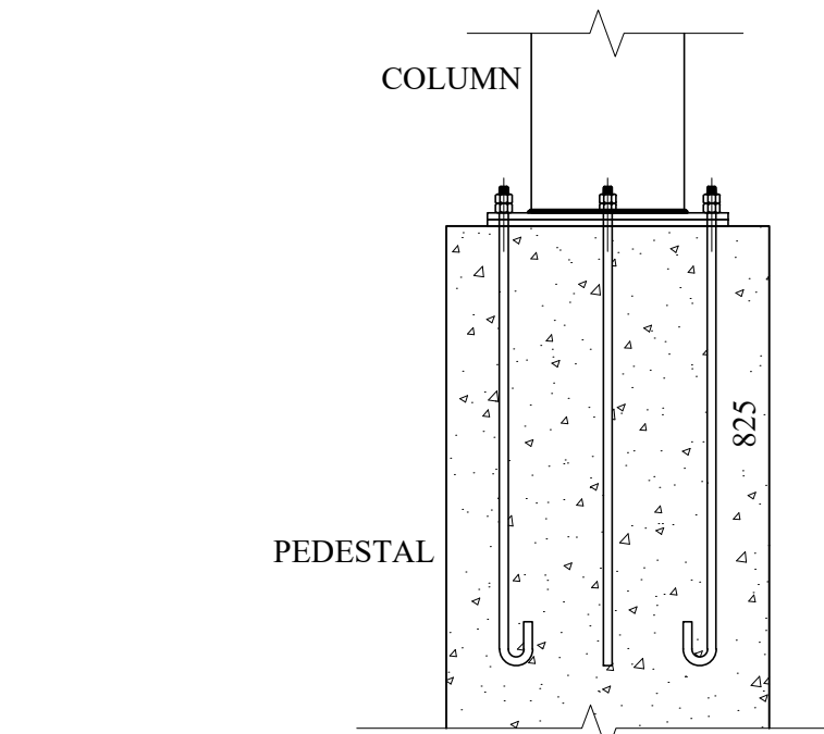
CONNECTION DETAILS FOR COLUMN AND FOUNDATION SCALE 1:20
