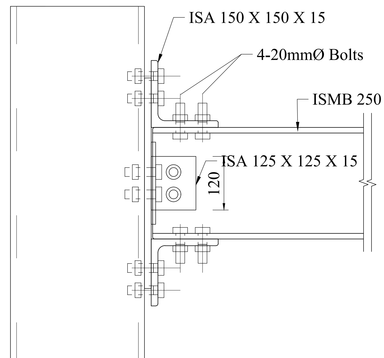
VIEW 1B-1
