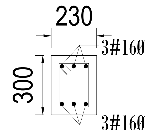
SECTION OF FOUNDATION BEAM (FB1)
