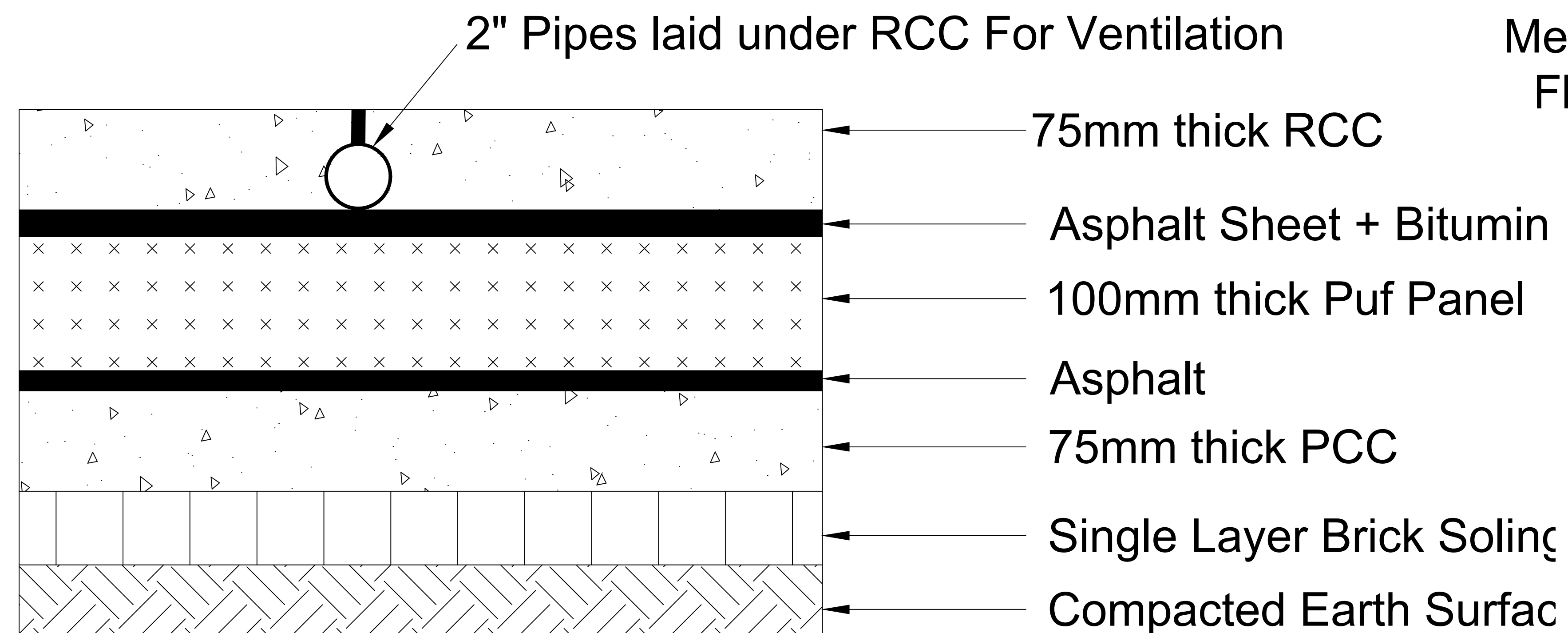
Ground Floor Detail
