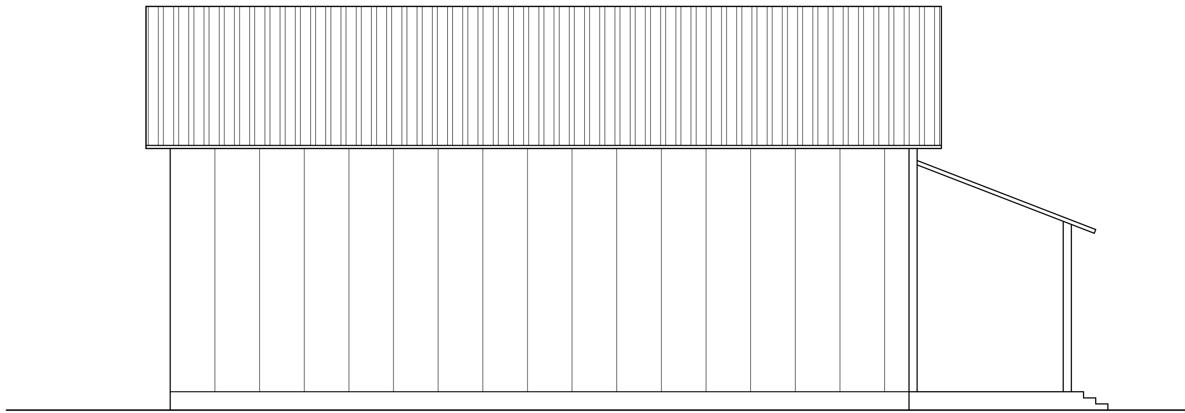
NORTH ELEVATION
