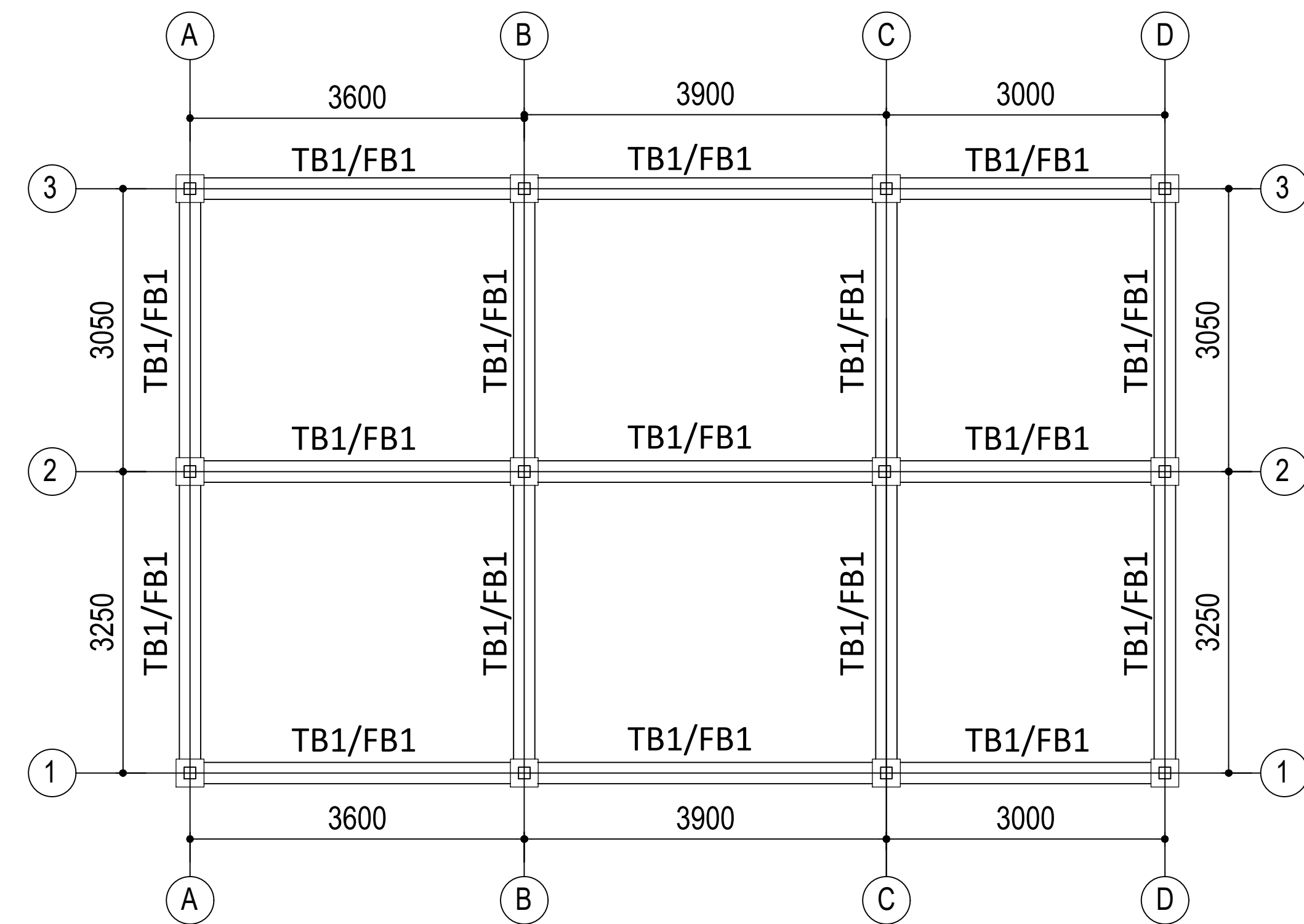
TIE BEAM LAYOUT PLAN
