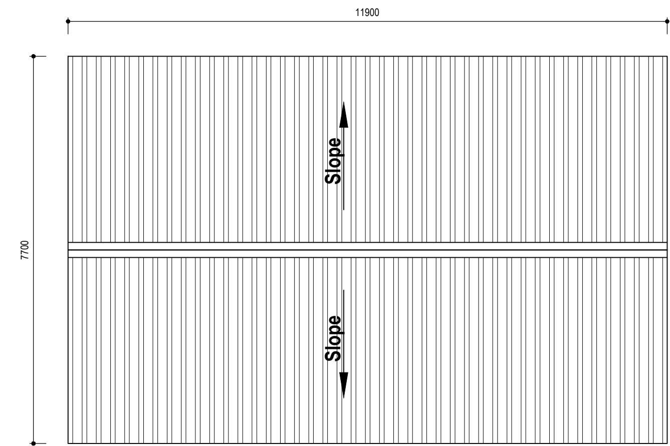
Roof Plan
