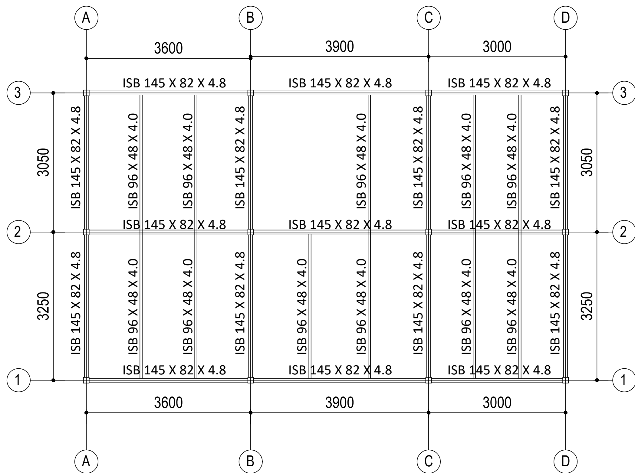
FIRST FLOOR BEAM LAYOUT PLAN
