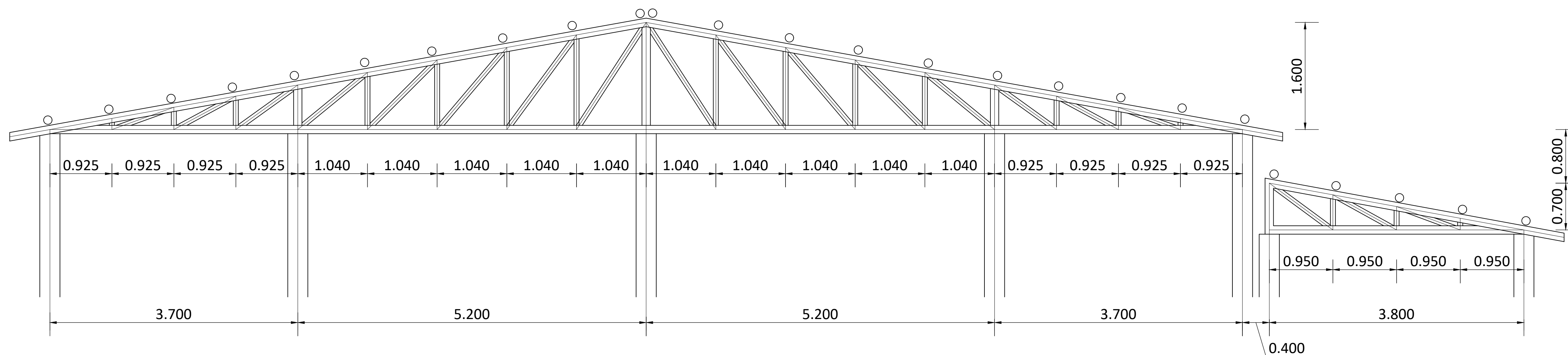
TRUSS ROOF ARRANGEMENT
