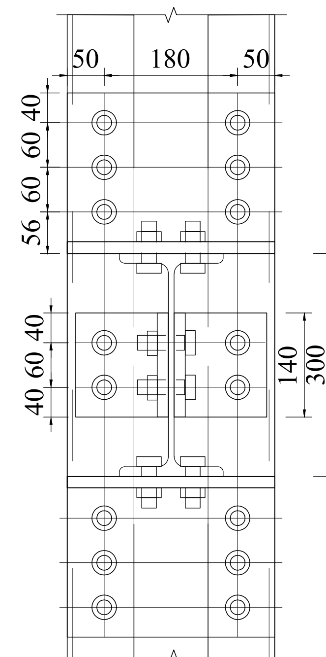
VIEW 3B-2
