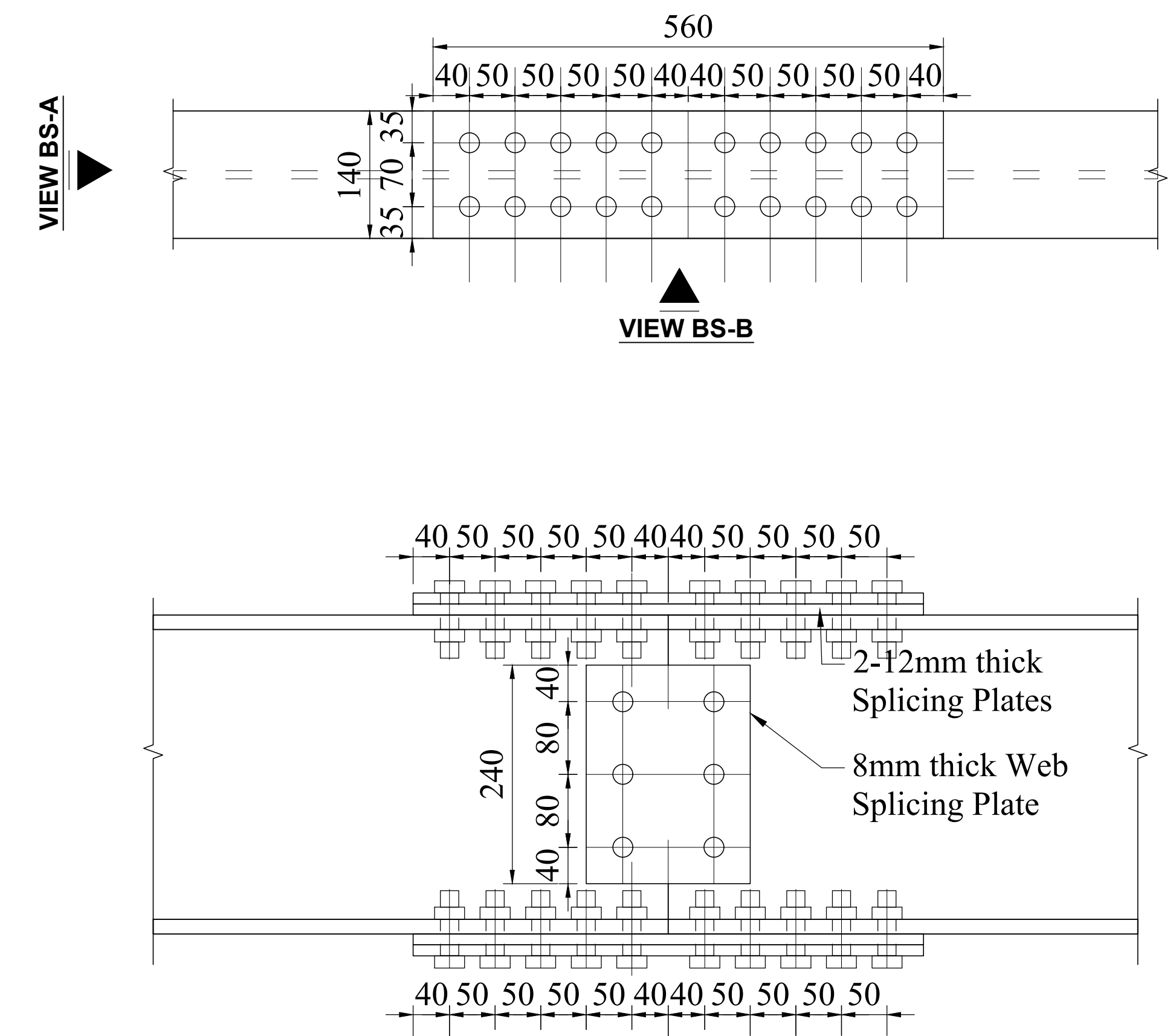
SPLICE FOR ISMB 350 SCALE 1:10
