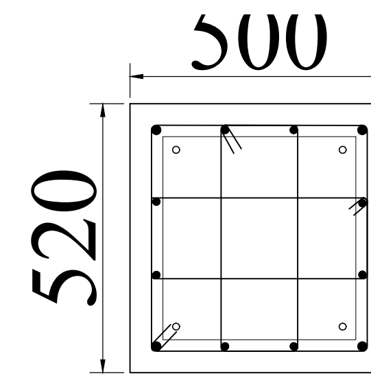
PEDESTAL DETAIL OF FOUNDATION-F1 and F2
