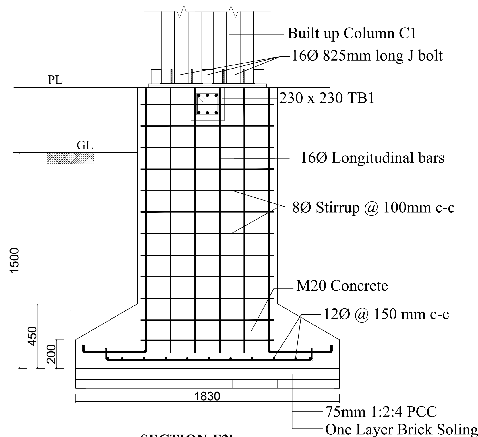
SECTION-F3b COLUMN FOUNDATION DETAILS
