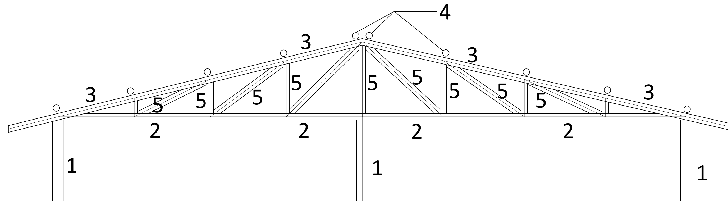
TRUSS MEMBER IDENTIFICATION
