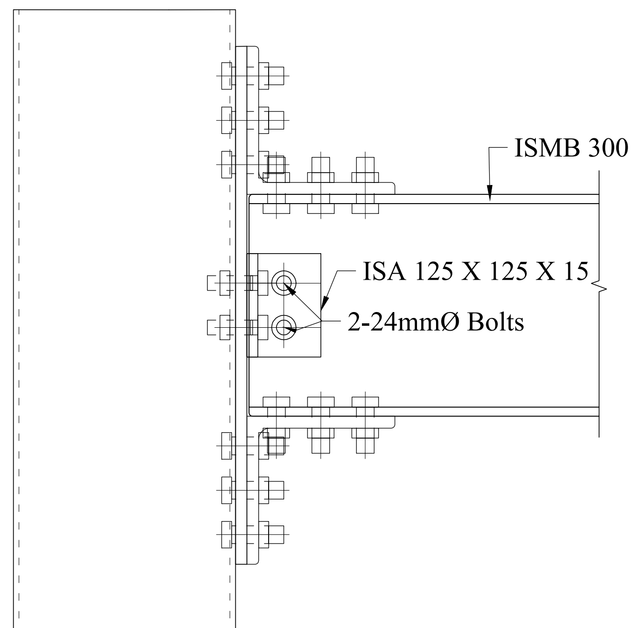
VIEW 2B-1
