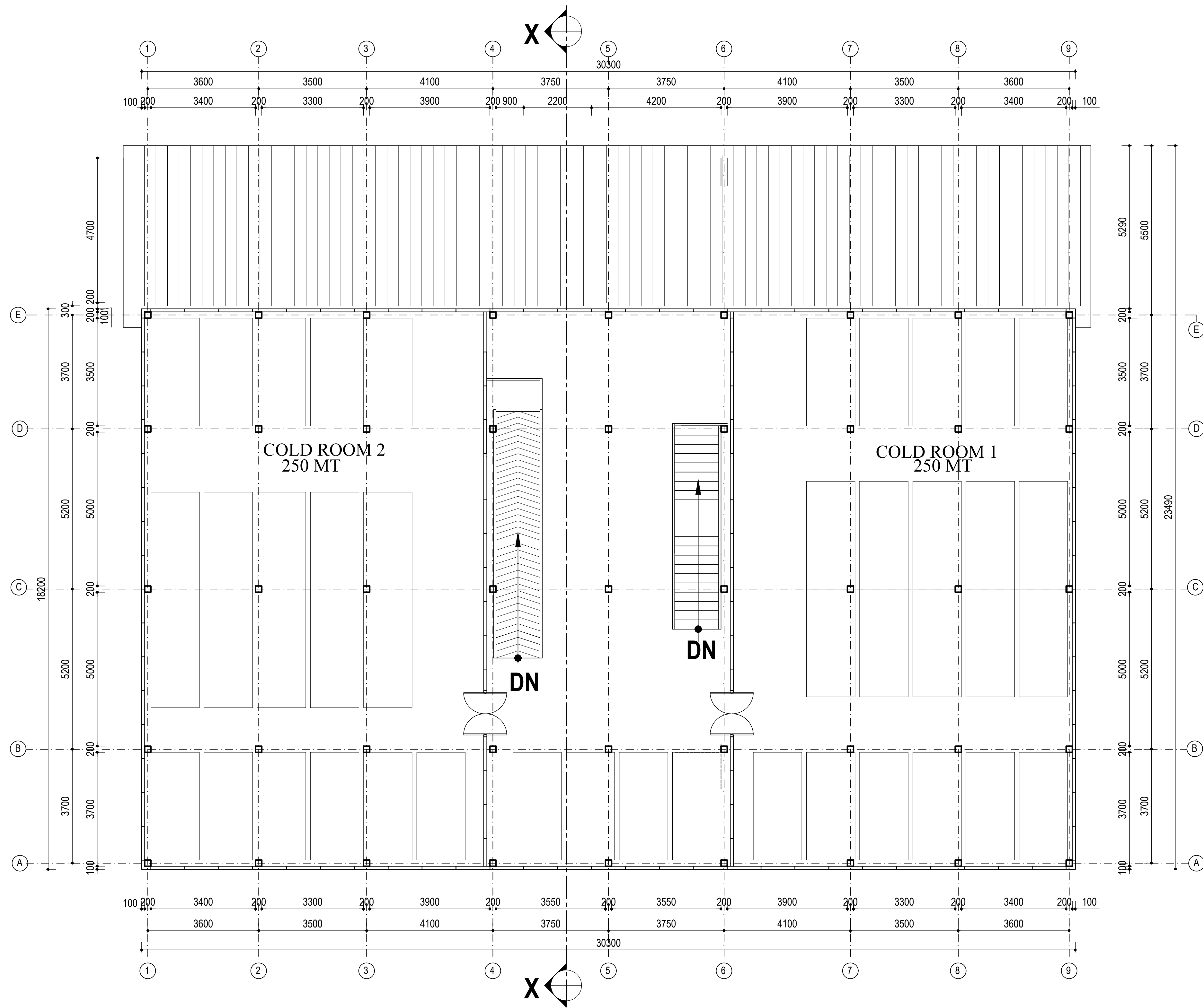
FIRST Floor Plan Floor Area: 551.4576 sq.m
