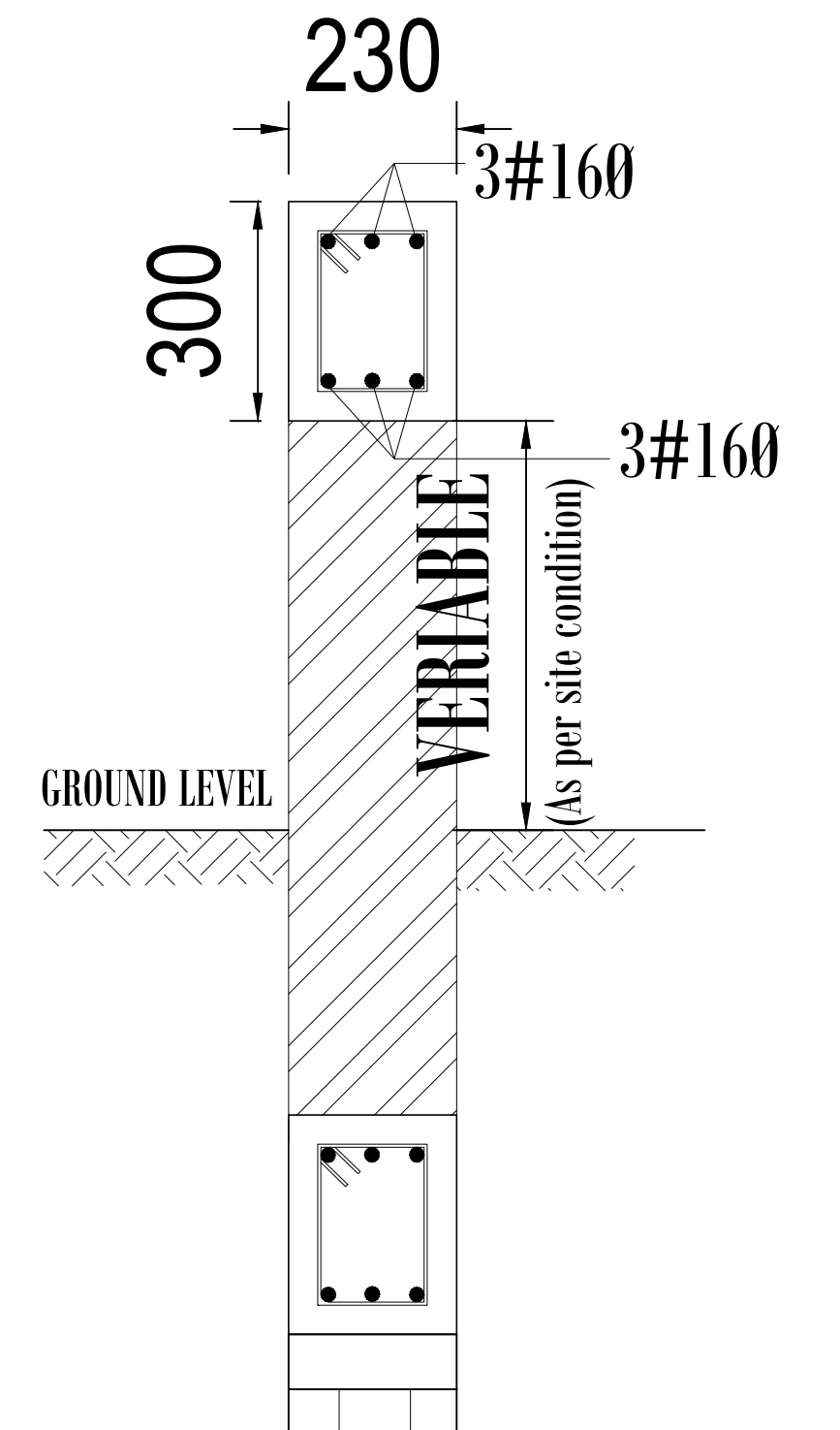
TOE WALL DETAIL
