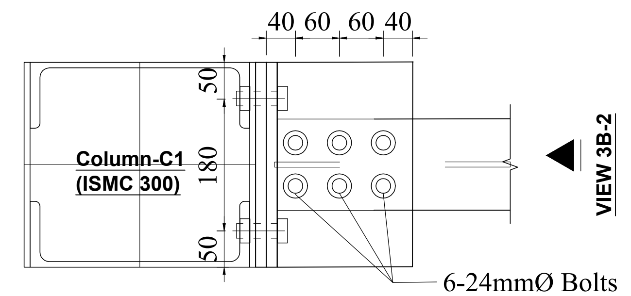
VIEW 3B-1
