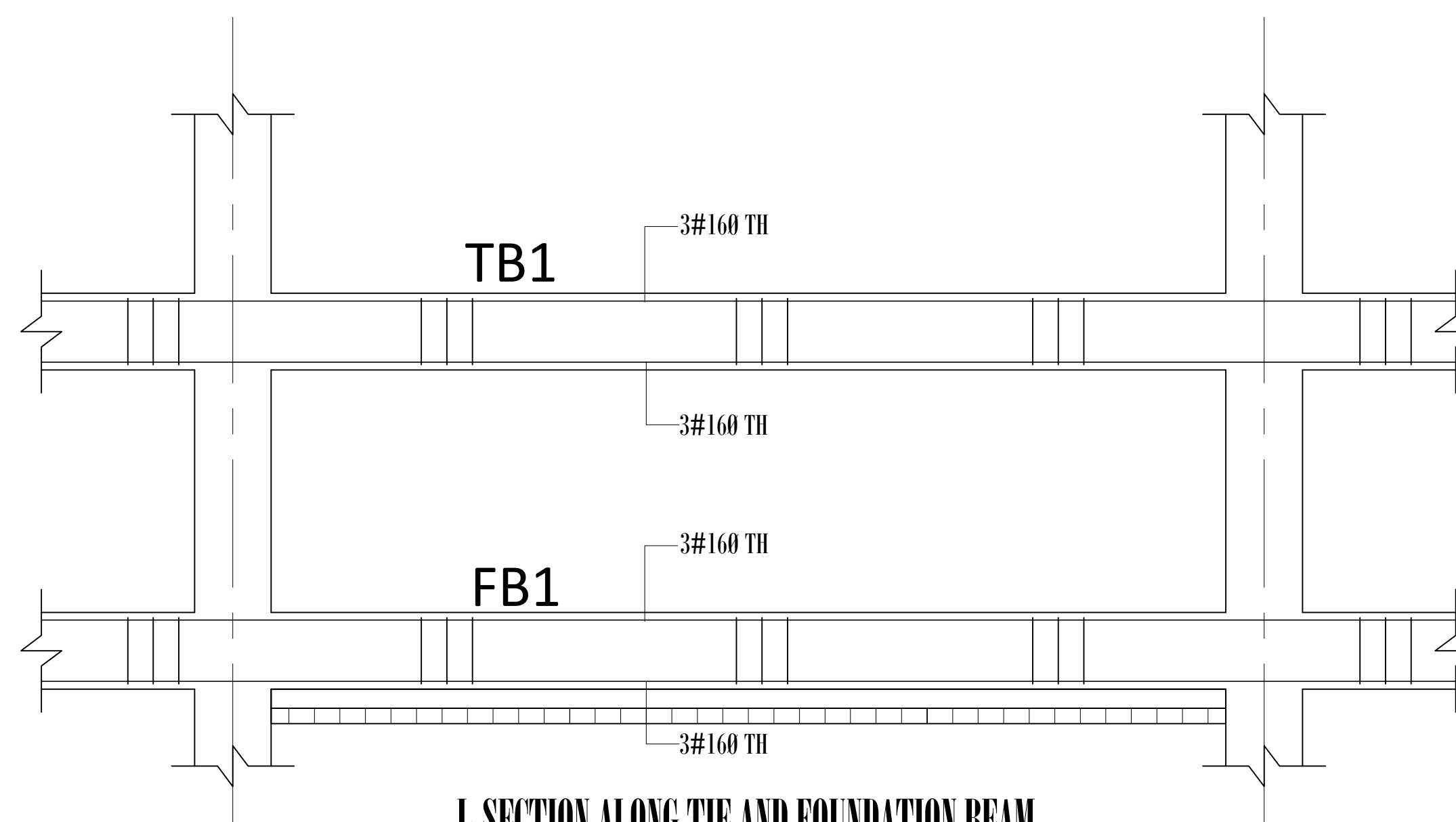
L-SECTION ALONG TIE AND FOUNDATION BEAM
