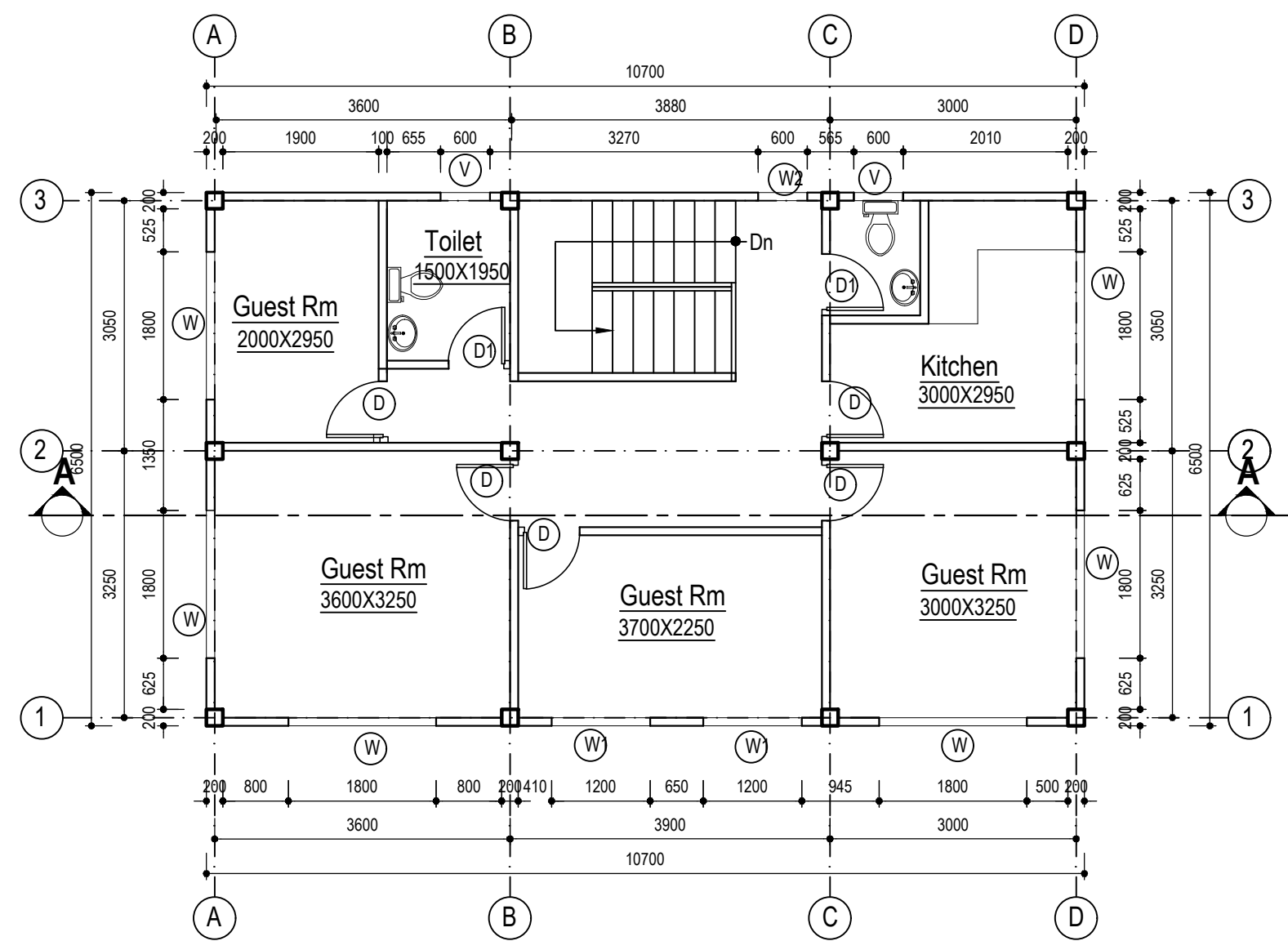
FIRST Floor Plan Floor Area:69.550 Sq.m
