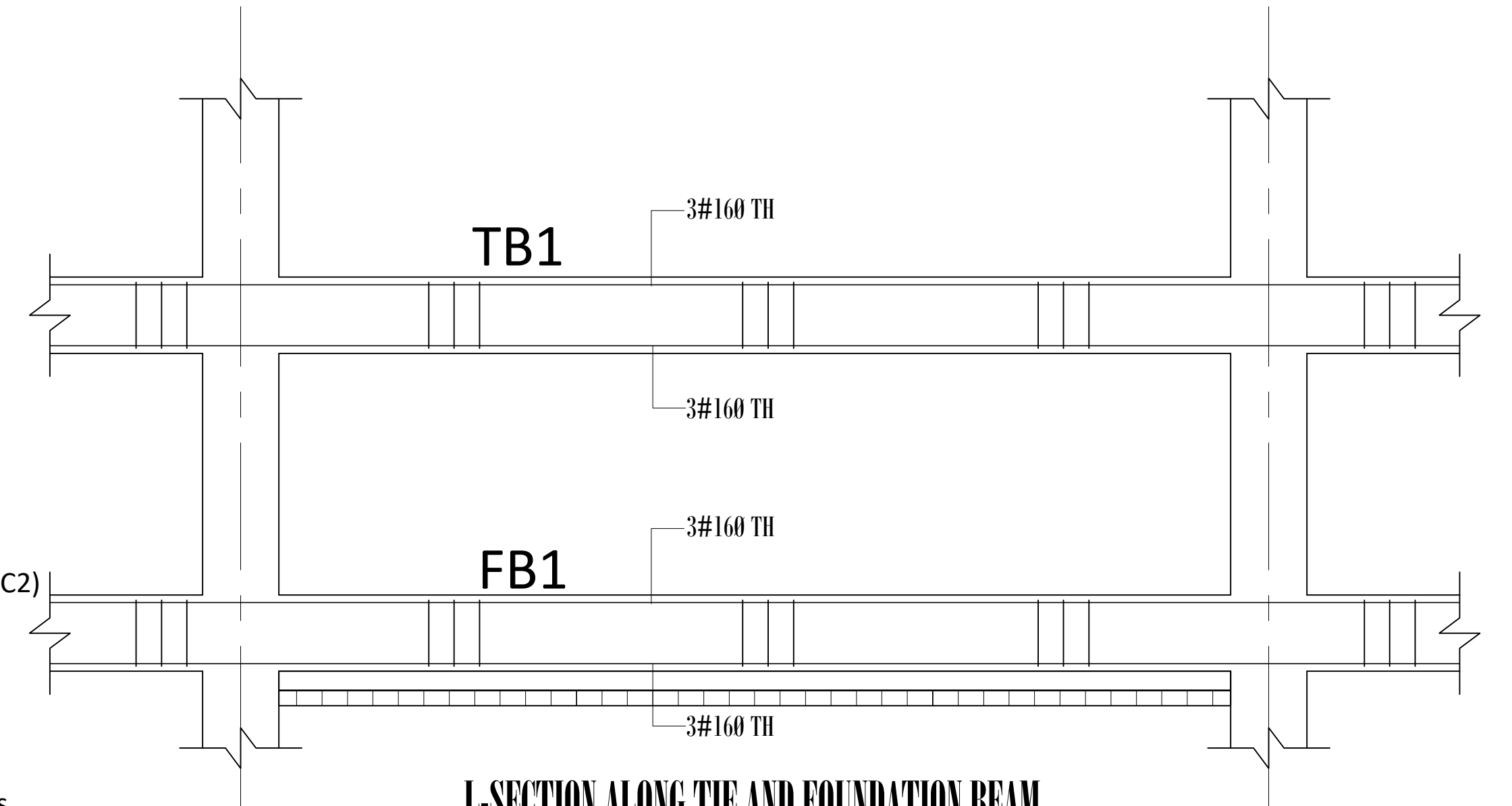
L-SECTION ALONG TIE AND FOUNDATION BEAM
