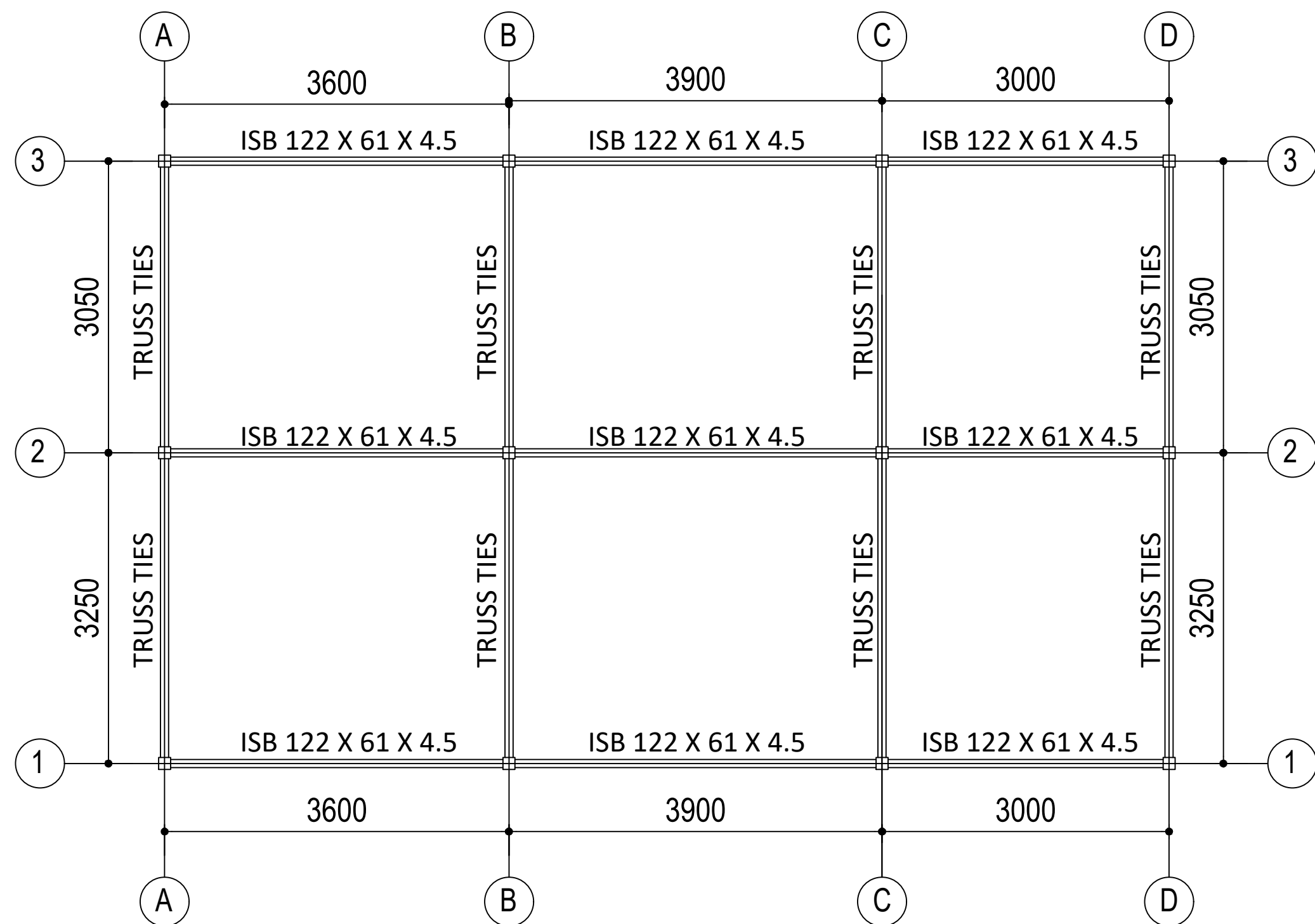
SECOND FLOOR BEAM LAYOUT PLAN
