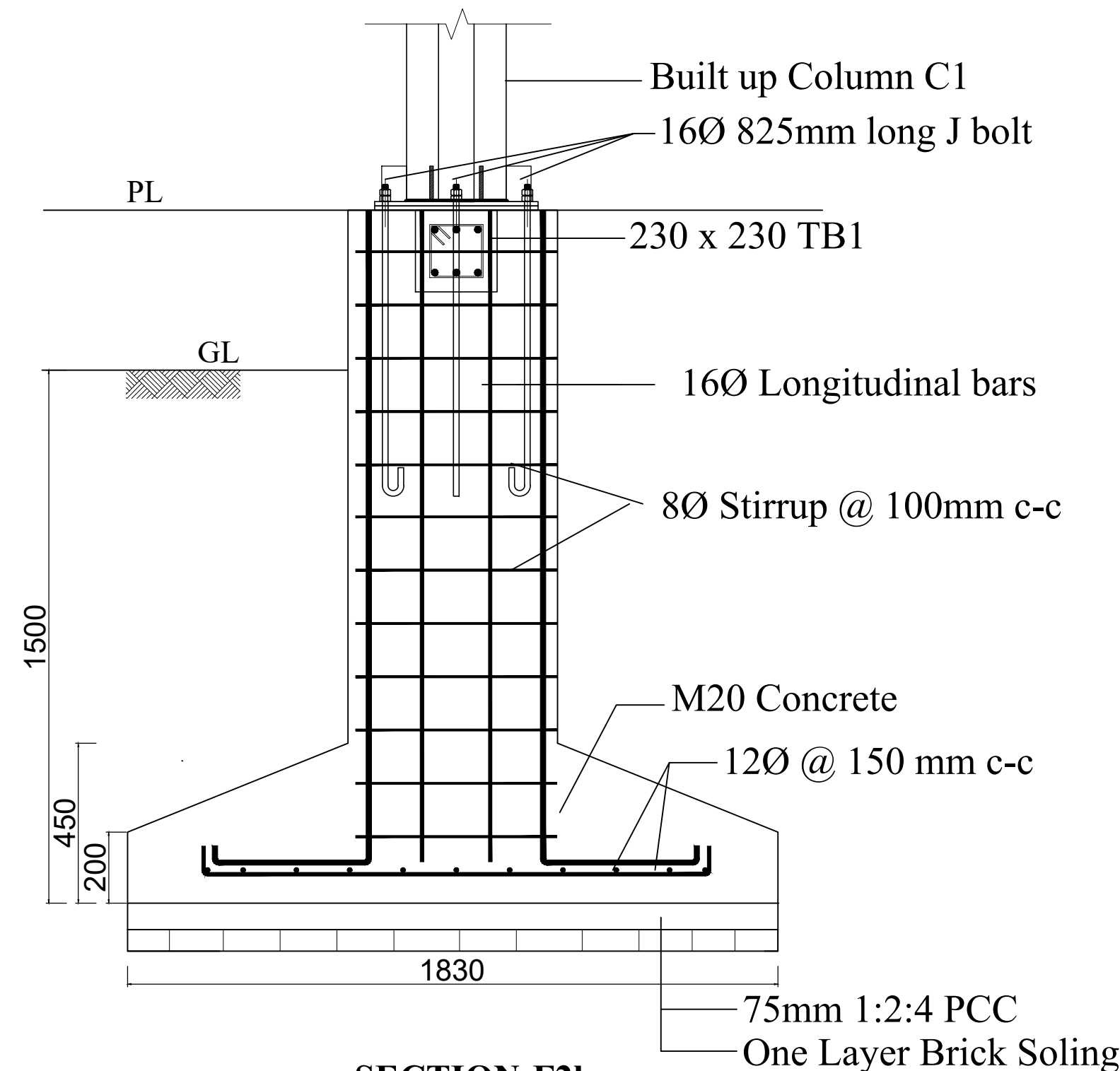
SECTION-F2b COLUMN FOUNDATION DETAILS
