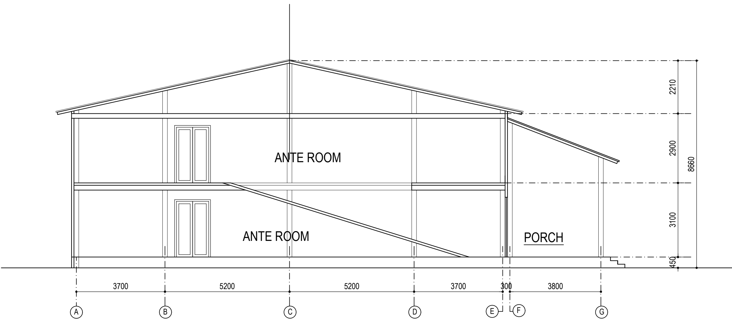
SECTION AT X-X
