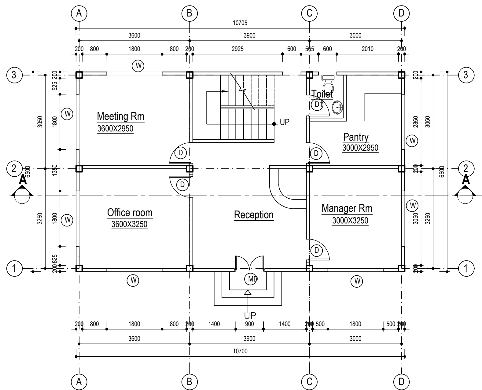
Ground Floor Plan Floor Area:69.550 Sq.m
