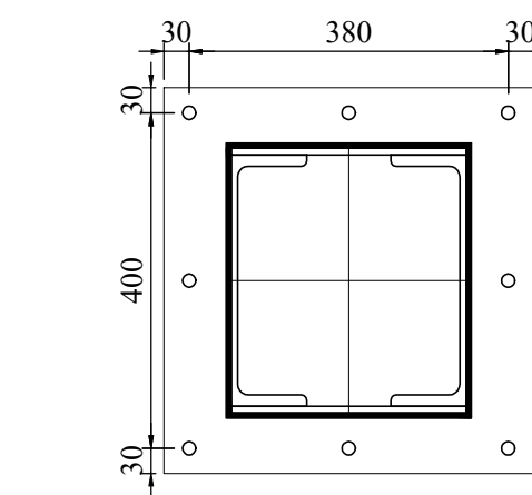
CONNECTION OF COLUMN & BASE PLATE
