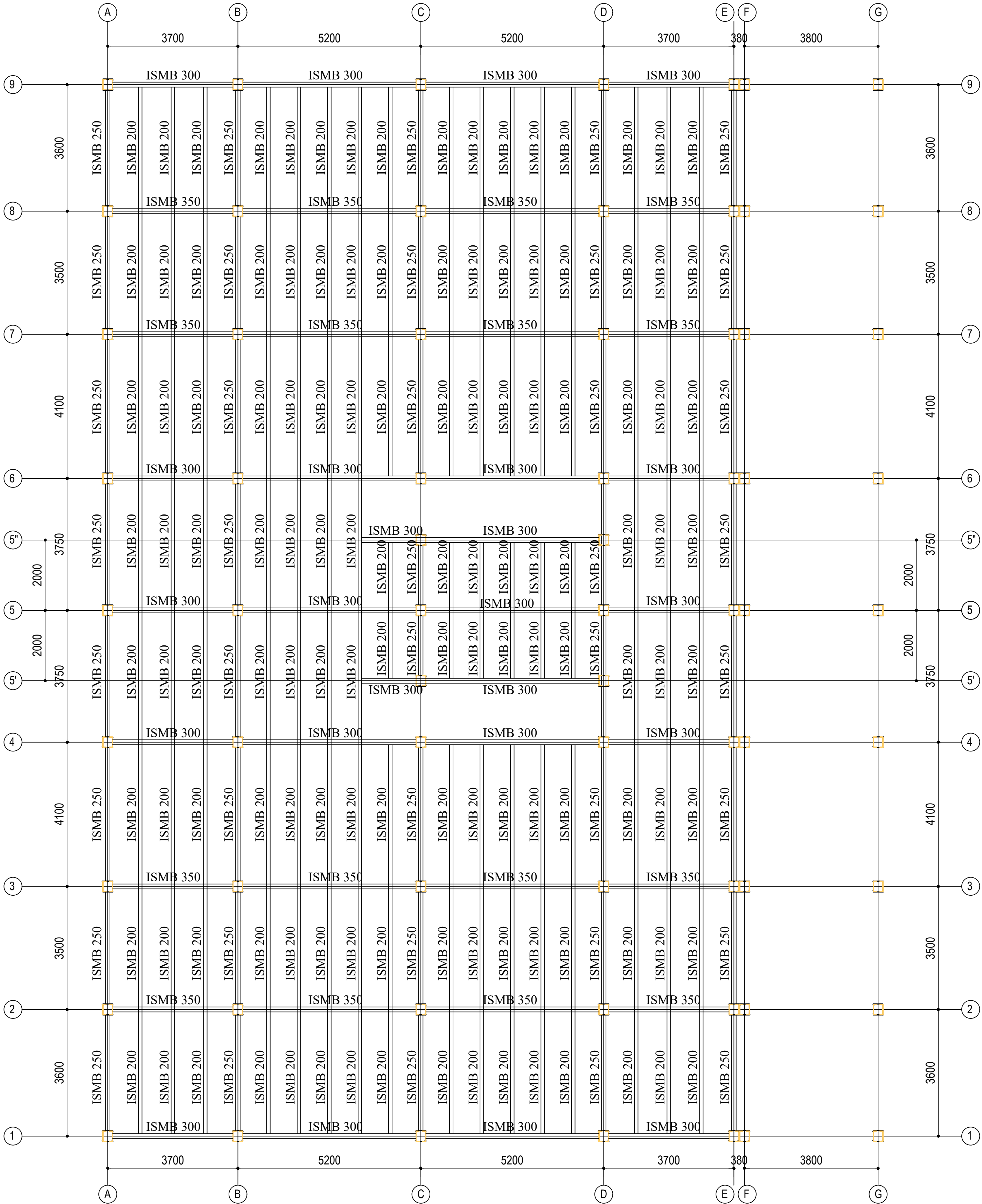
First Floor Beam Layout Plan
