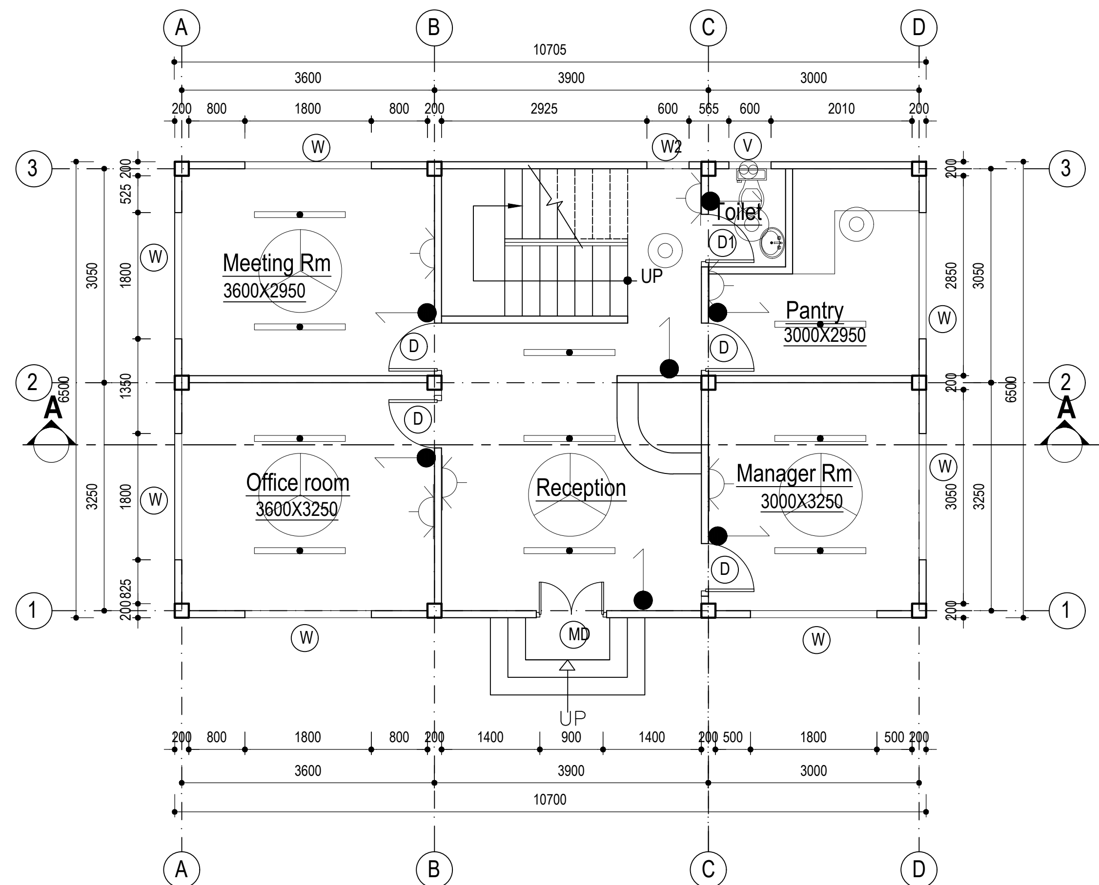
Ground Floor Plan Floor Area:69.550 Sq.m
