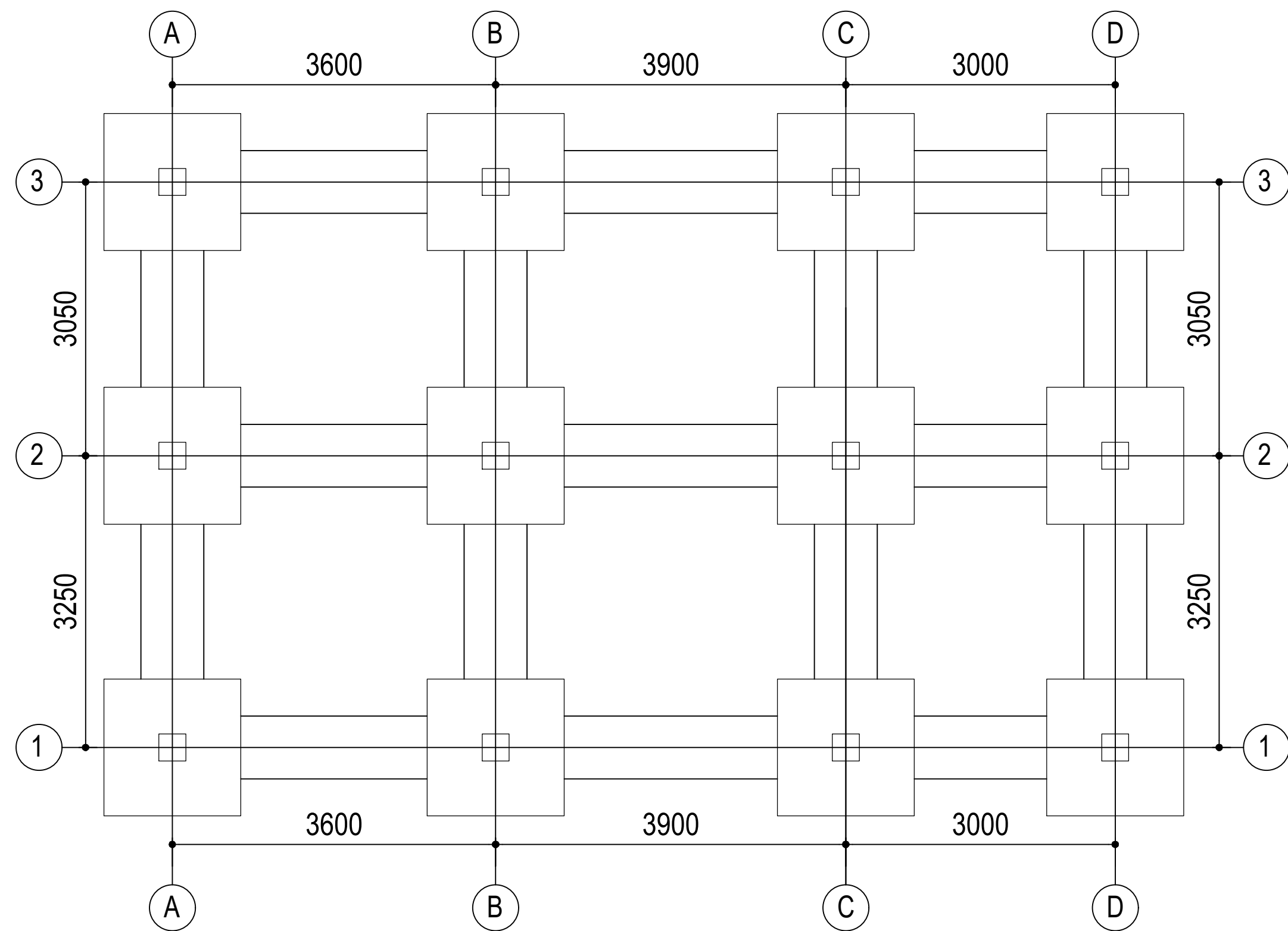
FOOTING TRENCH PLAN
