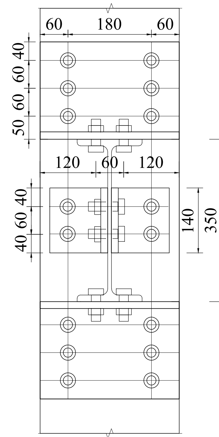
VIEW 3A-2
