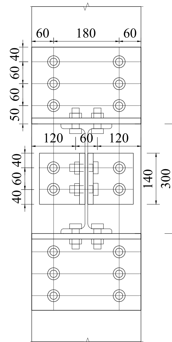
VIEW 2A-2
