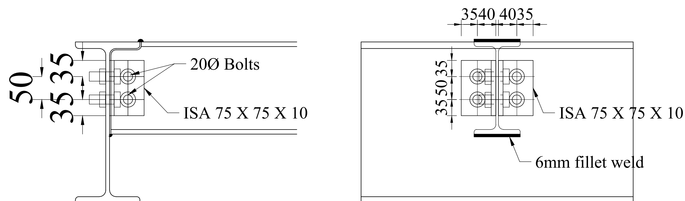
Beam - Beam Connection
