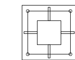
BASE PLATE DETAIL (285x285x12) (For Vertical Post - C2)
