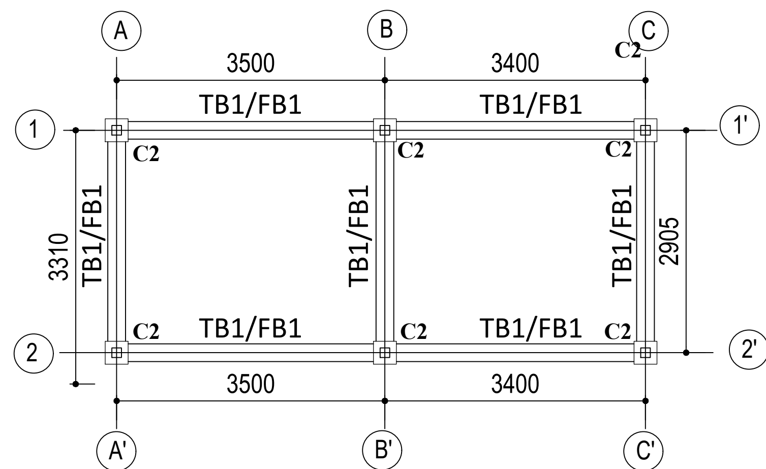
TIE BEAM LAYOUT PLAN
