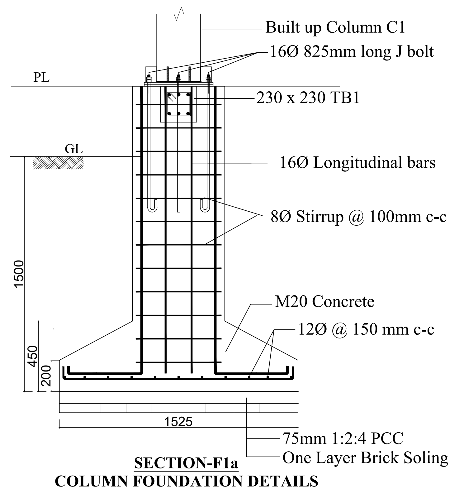
FOUNDATION-F1
