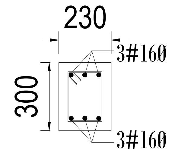
SECTION OF TIE BEAM (TB1)
