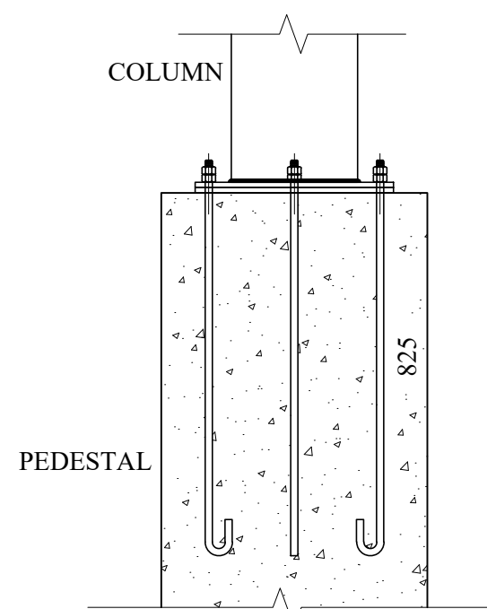
CONNECTION DETAILS FOR COLUMN AND FOUNDATION SCALE 1:20
