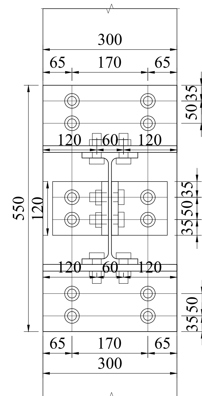
VIEW 1A-2
