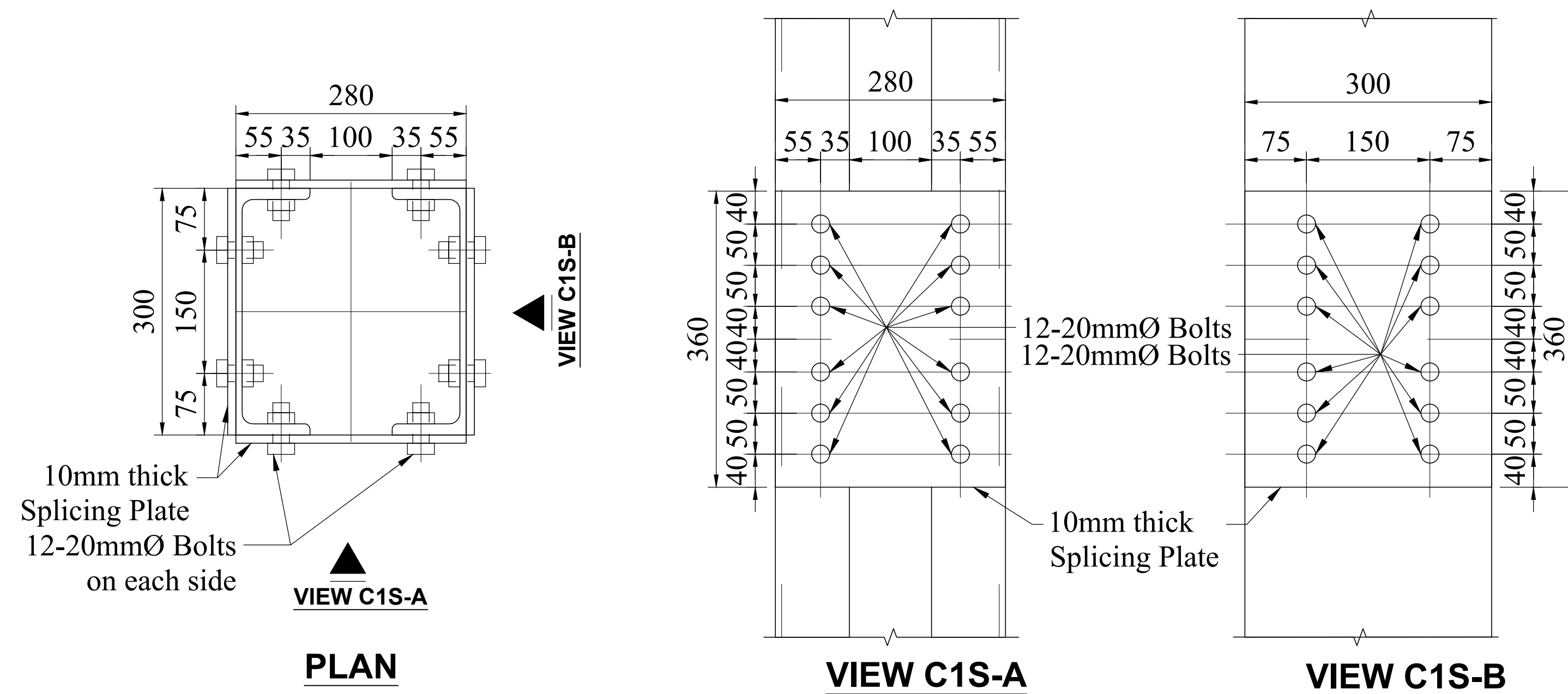
SPLICE FOR COLUMN-C1
