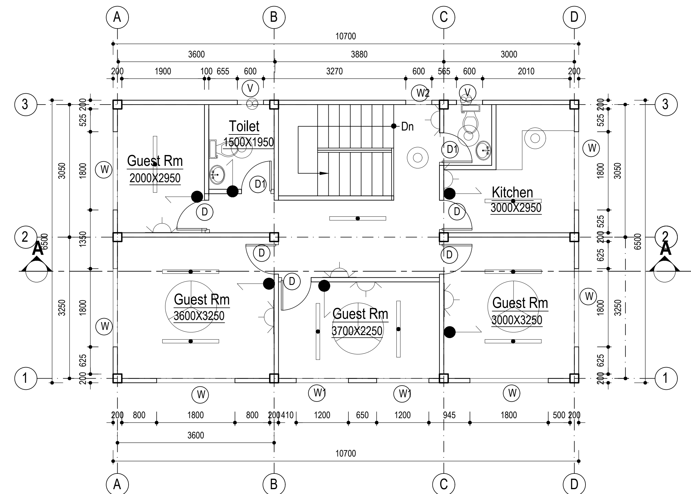
FIRST Floor Plan Floor Area:69.550 Sq.m
