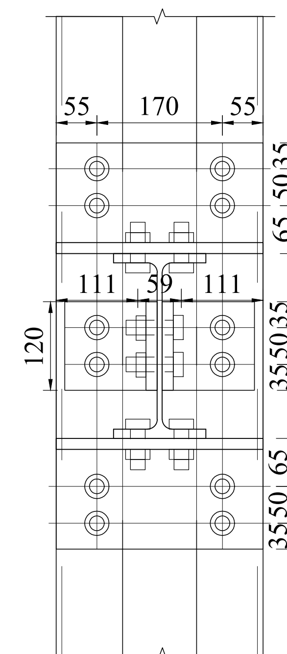
VIEW 1B-2
