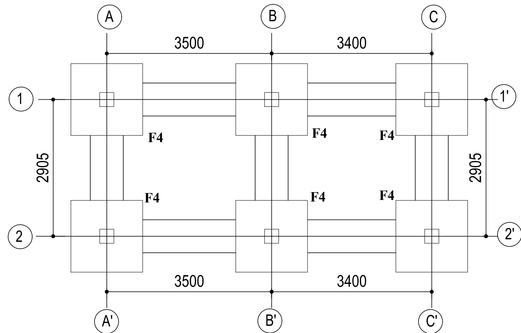
FOOTING TRENCH PLAN
