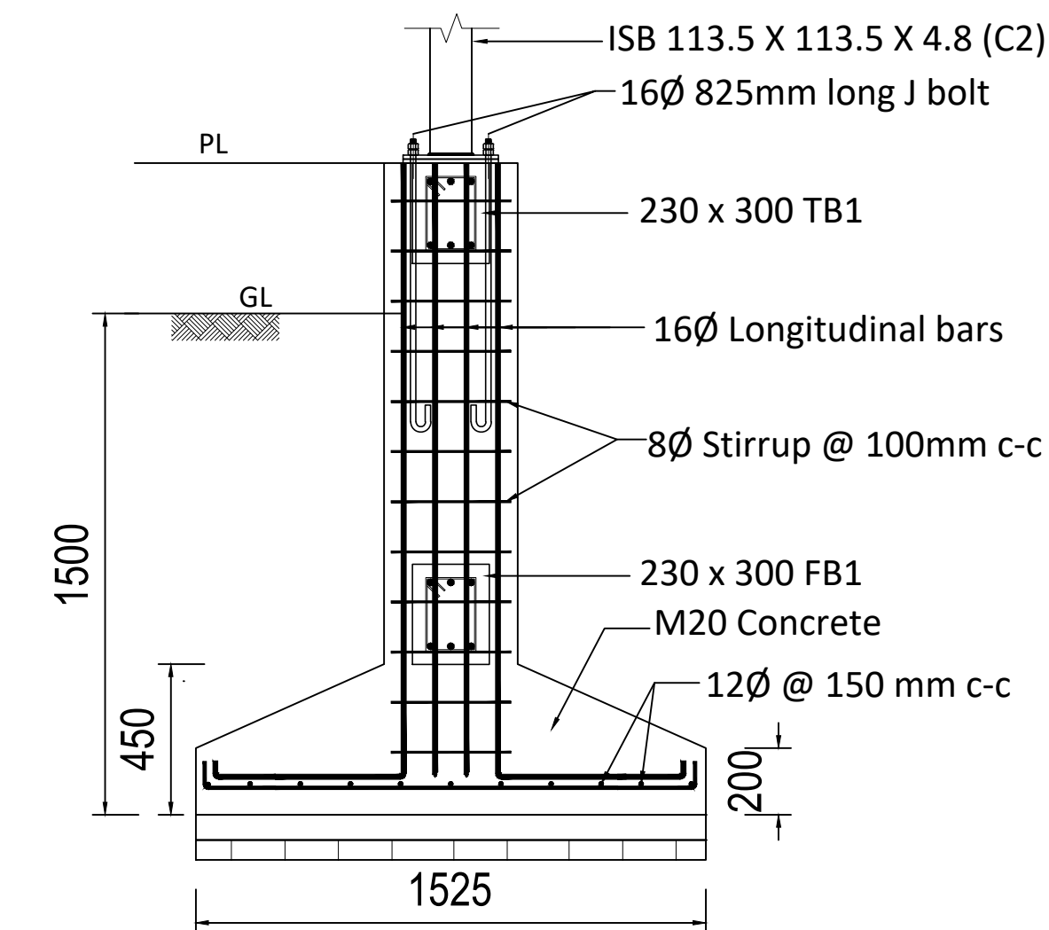
SECTION OF FOUNDATION-F4
