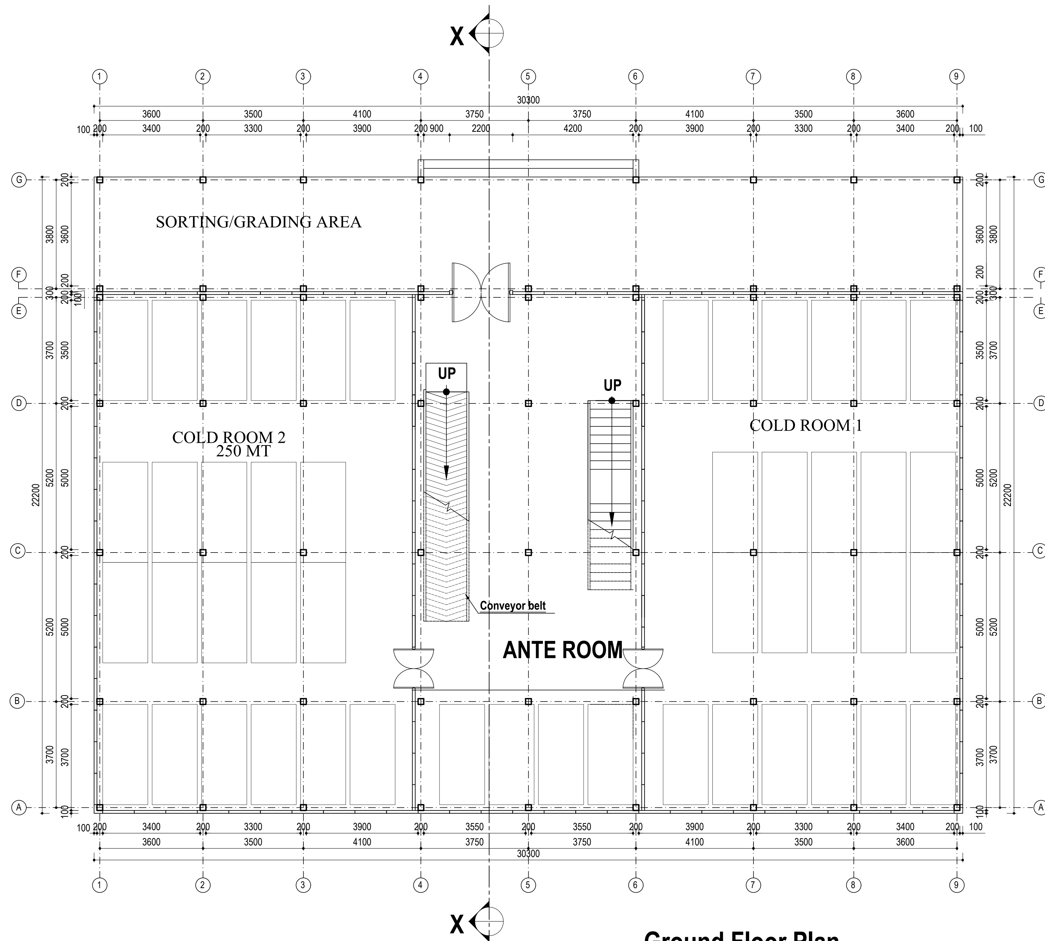
Ground Floor Plan Floor Area:672.660 sq.m
