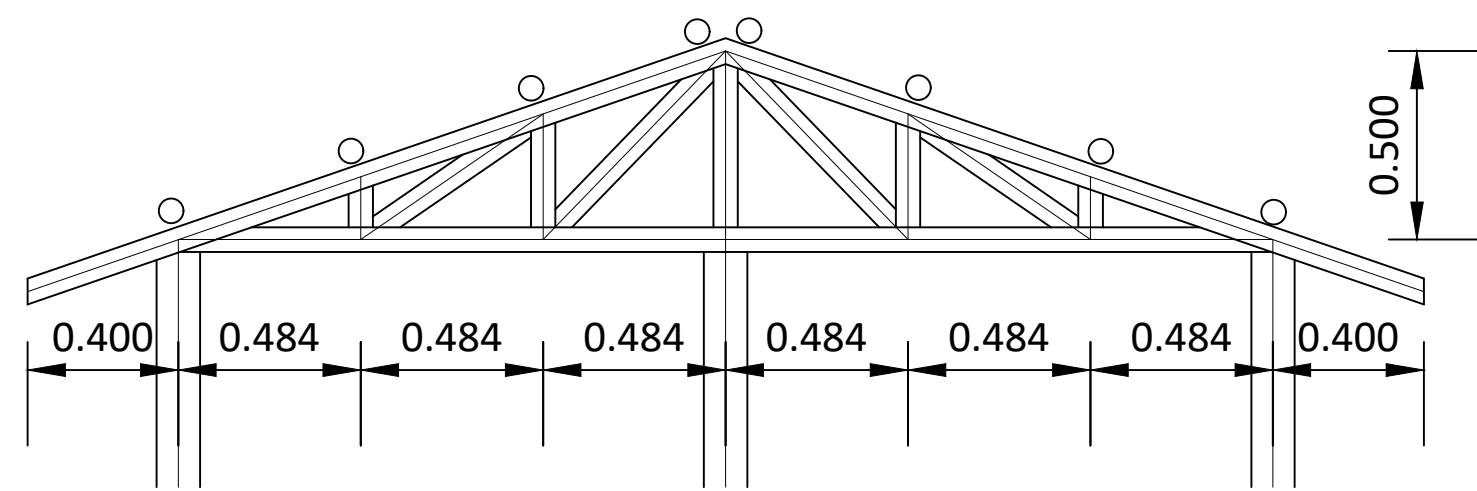
TRUSS MEMBER SIZES
