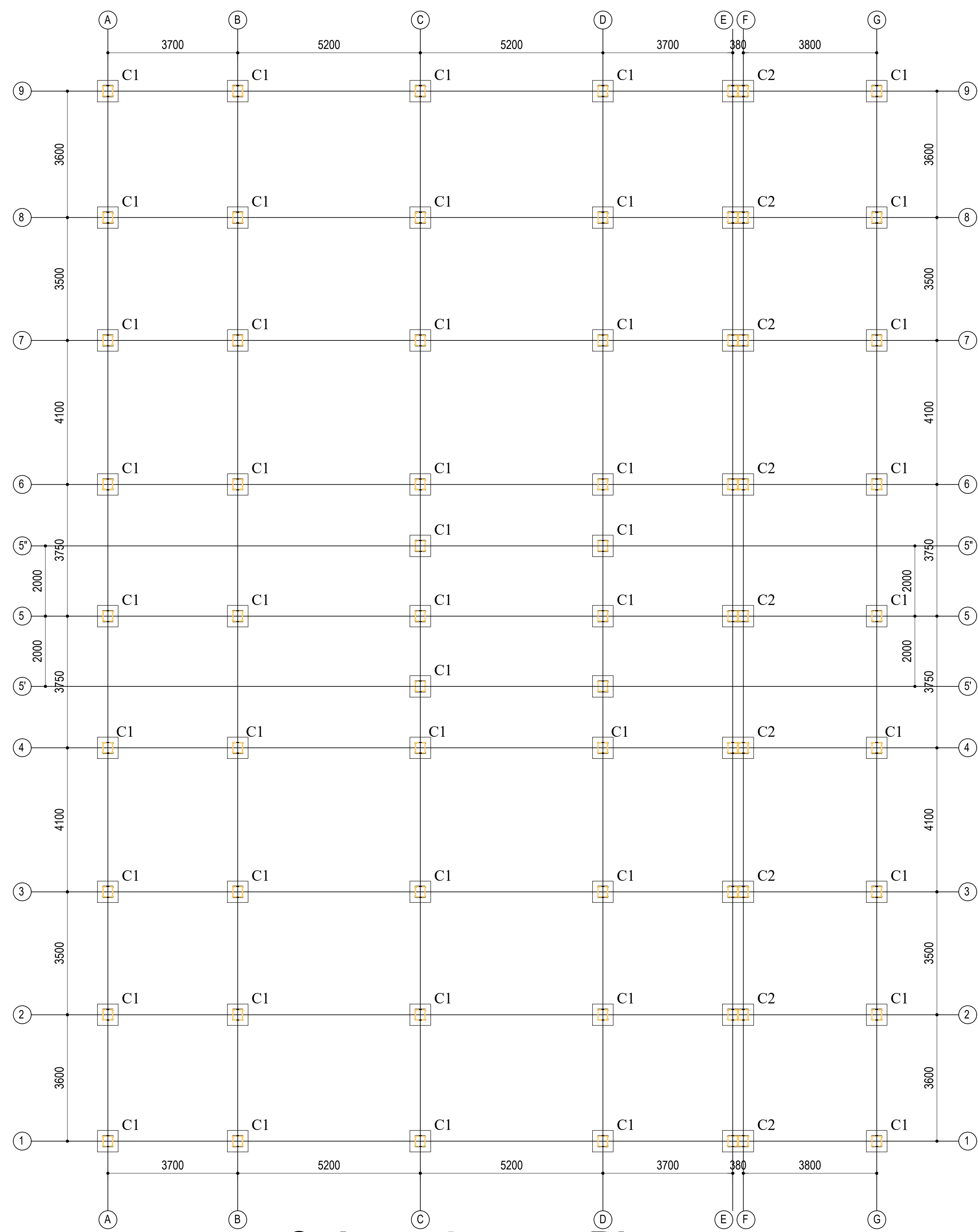
Column Layout Plan
