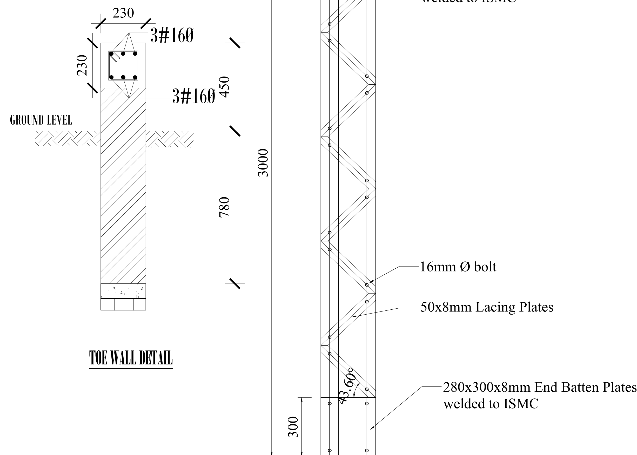
ELEVATION OF COLUMNS C1
