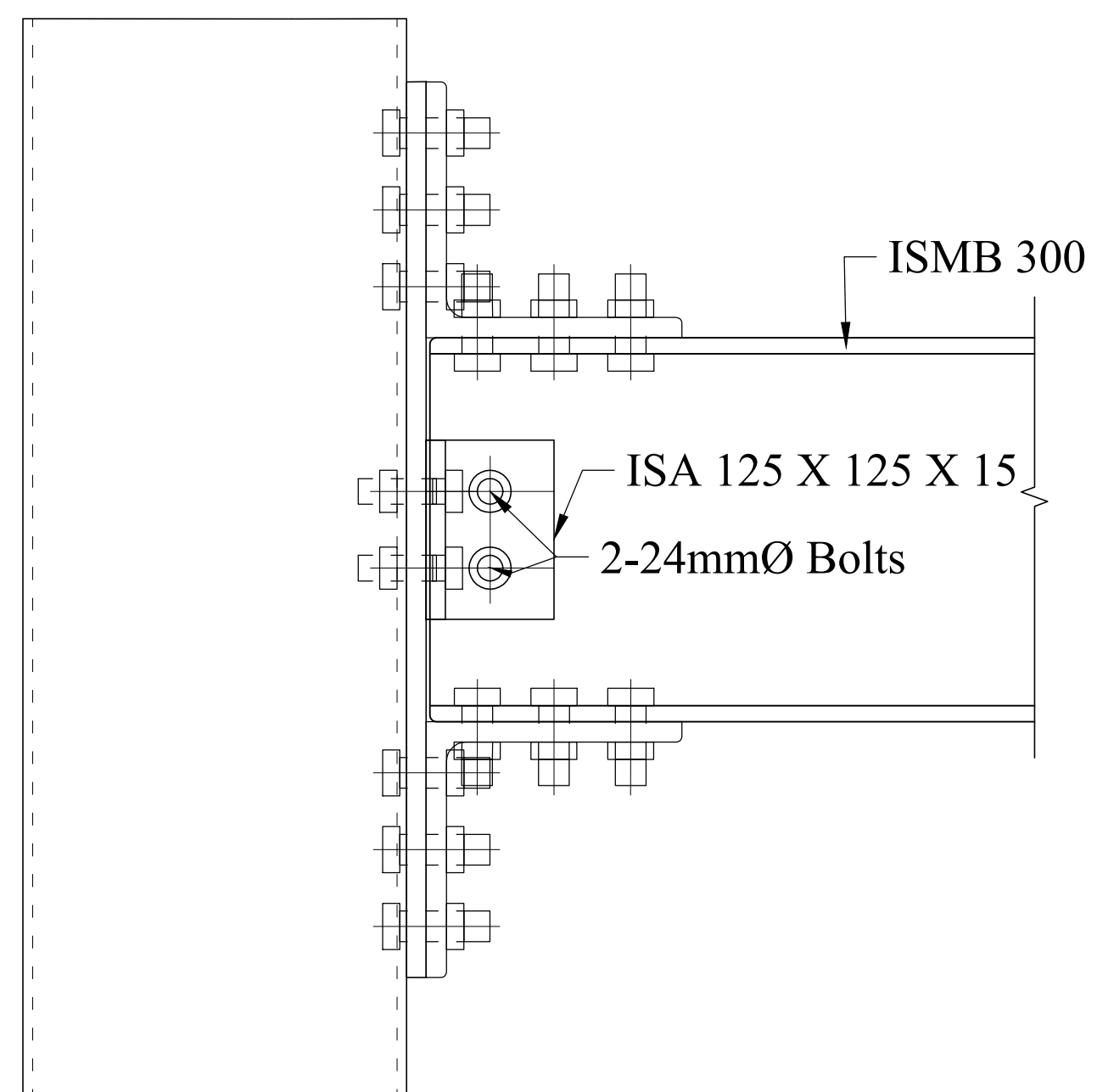
VIEW 3B-1
