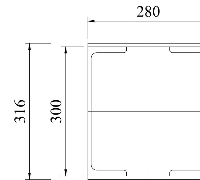
C1 ISMC 300
