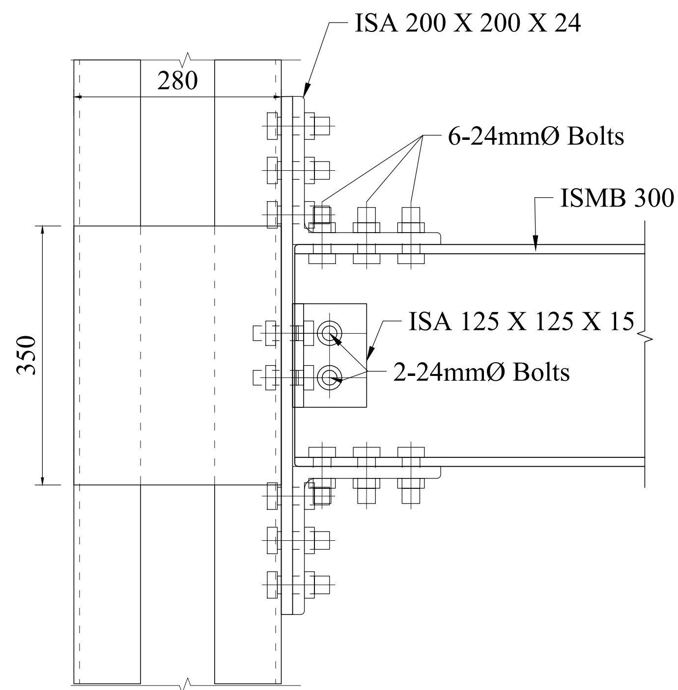
VIEW 2A-1
