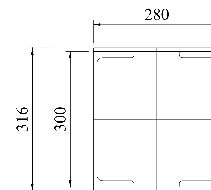
C1 ISMC 300
