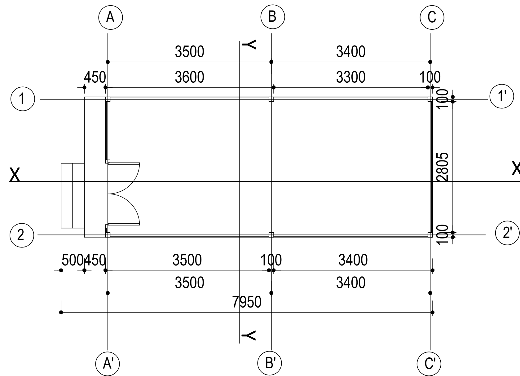
FLOOR PLAN
