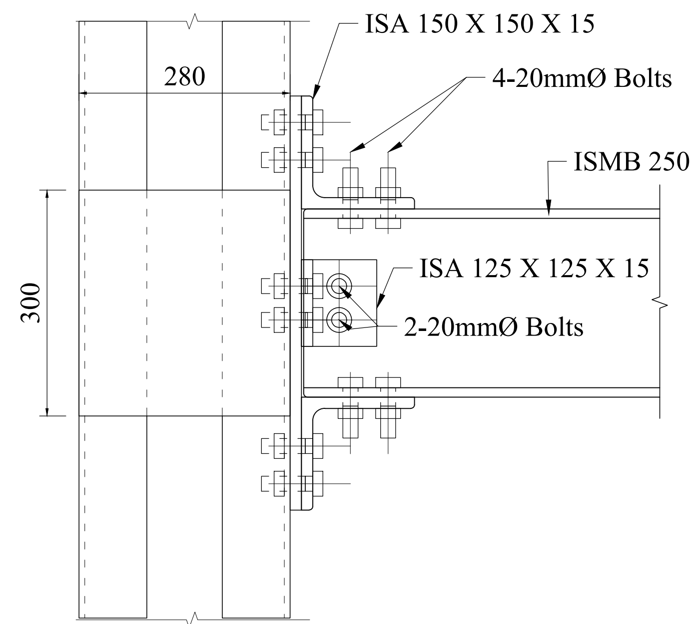
VIEW 1A-1
