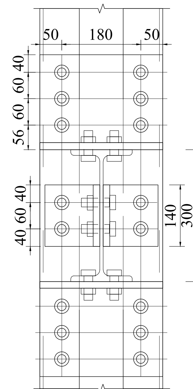
VIEW 2B-2
