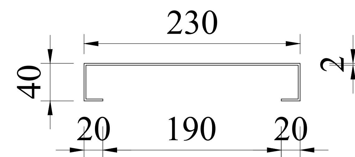
Mezzanine Perforated Flooring Unit Detail
